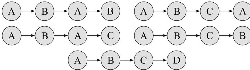
Figure 1: Motifs of size four.
